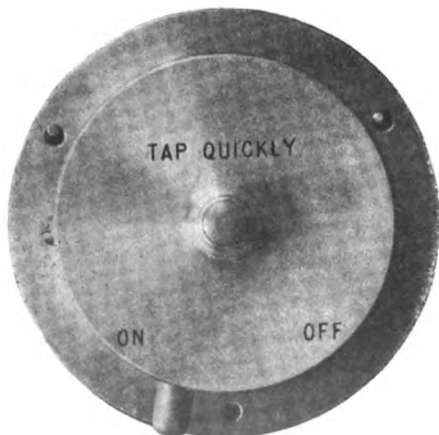
SIMMS DASHBOARD STARTING SWITCH.
